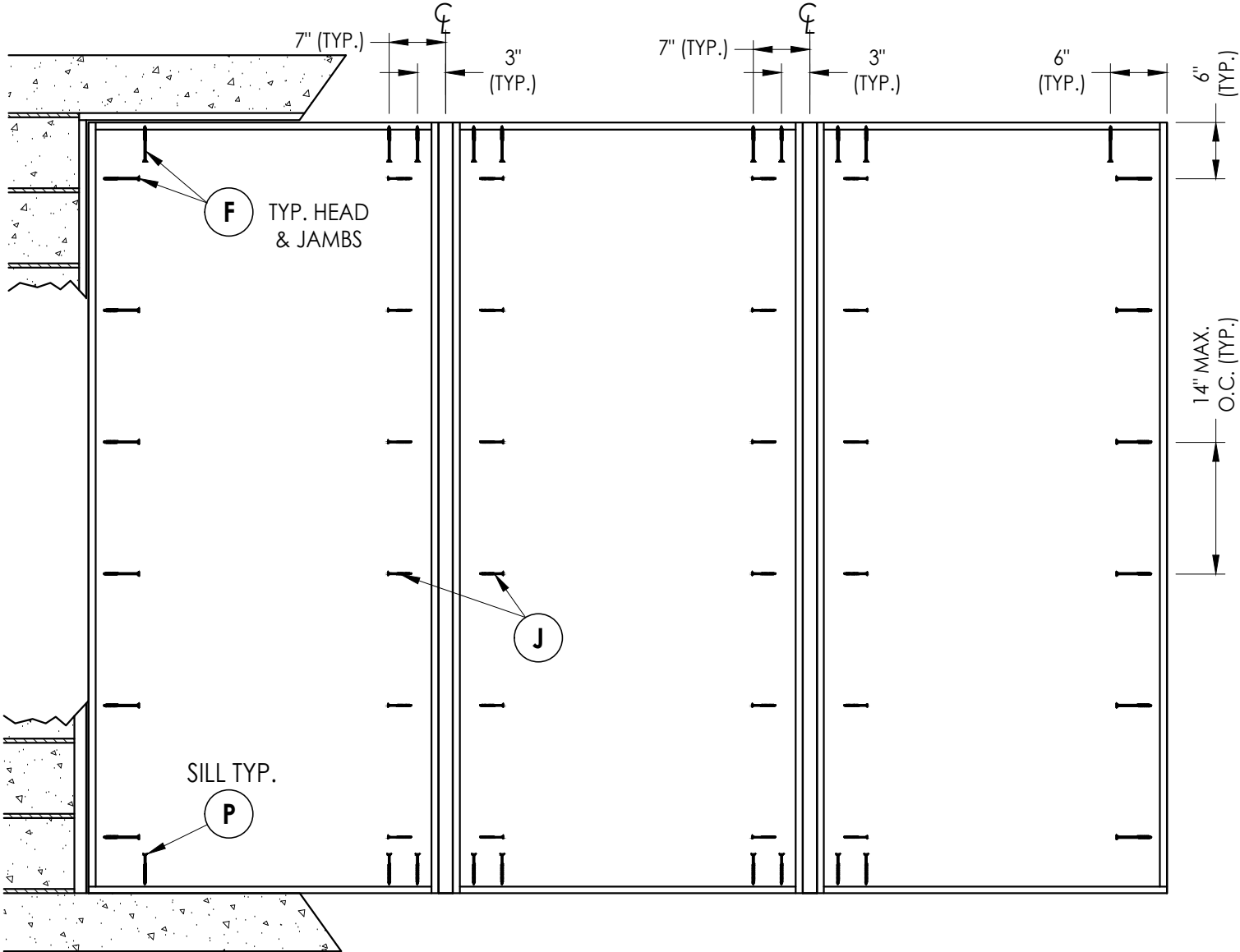
FRAME ANCHORING Masonry 1X buck construction
