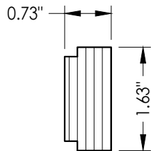
36 LITE OPENING STILE REINF.
