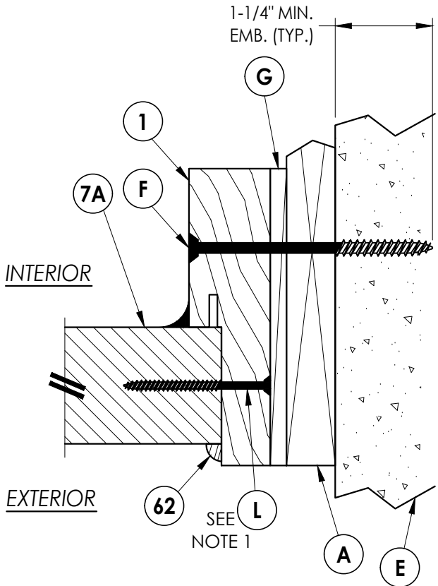
3/4 HORIZONTAL CROSS SECTION Shown w/1X sub-buck
